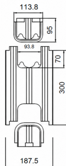
VISTA FRONTAL
