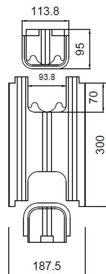
VISTA FRONTAL
